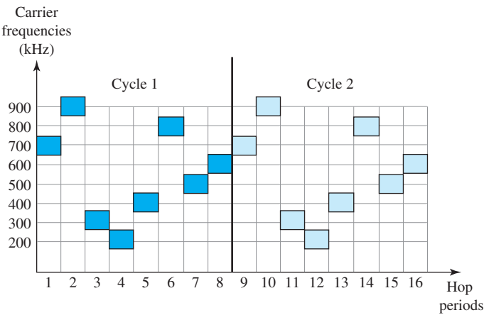
Figure 6.30 FHSS cycles
