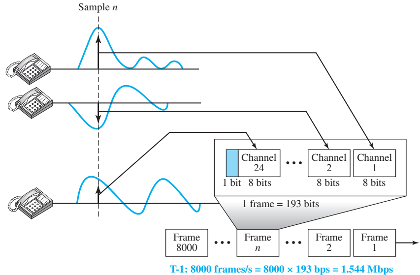
Figure 6.25 T-1 frame structure
