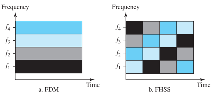
Figure 6.31 Bandwidth sharing
